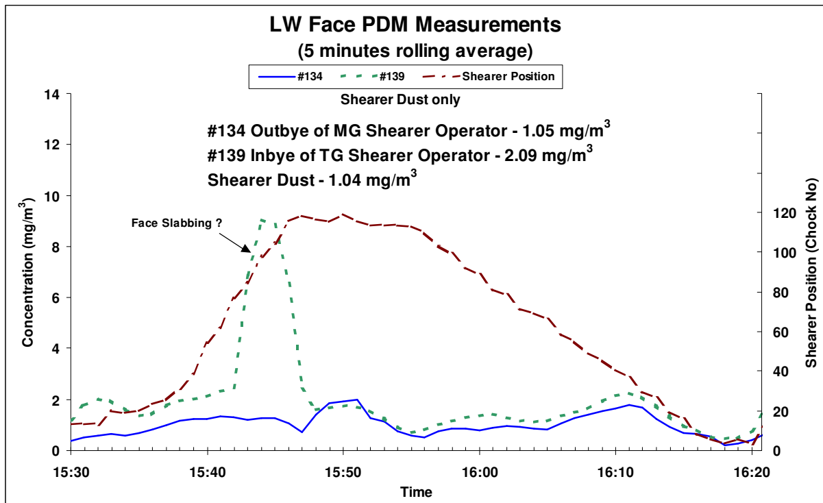
Figure 15 Relative dust make experienced at MG end of the face and the operator position closest to the TG.
