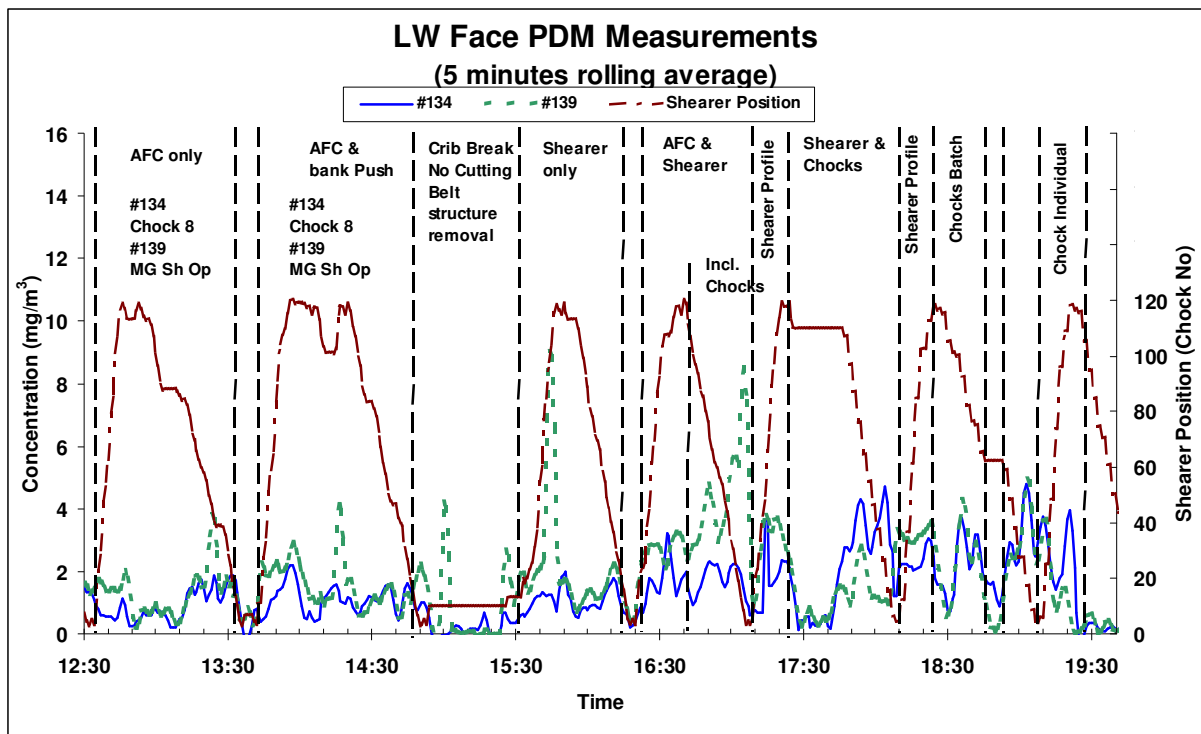
Figure 11 LW Face Dust Surveys Shearer Position and dust monitored points m Levels
