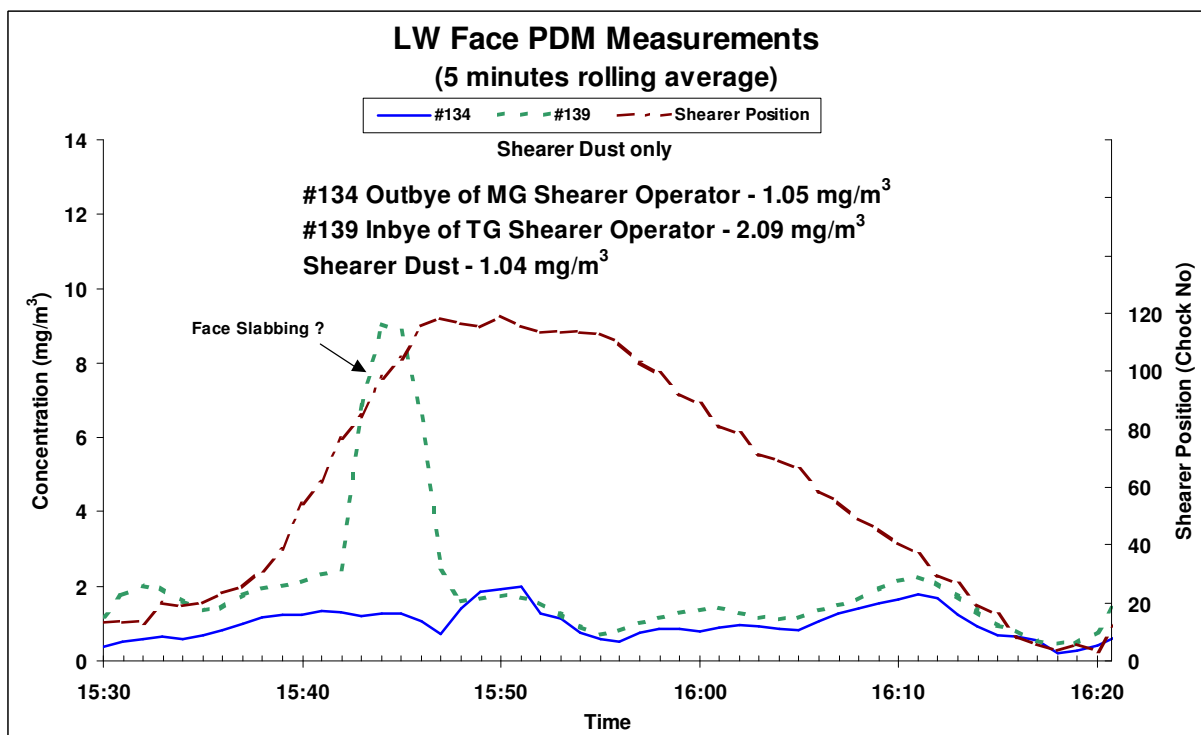
Figure 12 Relative dust make experienced by MG and TG shearer operators.
