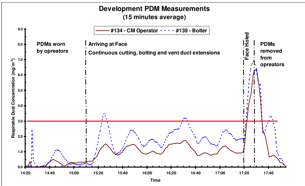
Figure 6 Development Face PDM results.
