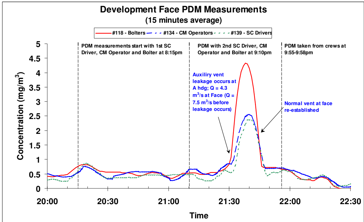
Figure 5 Development Face PDM results.
