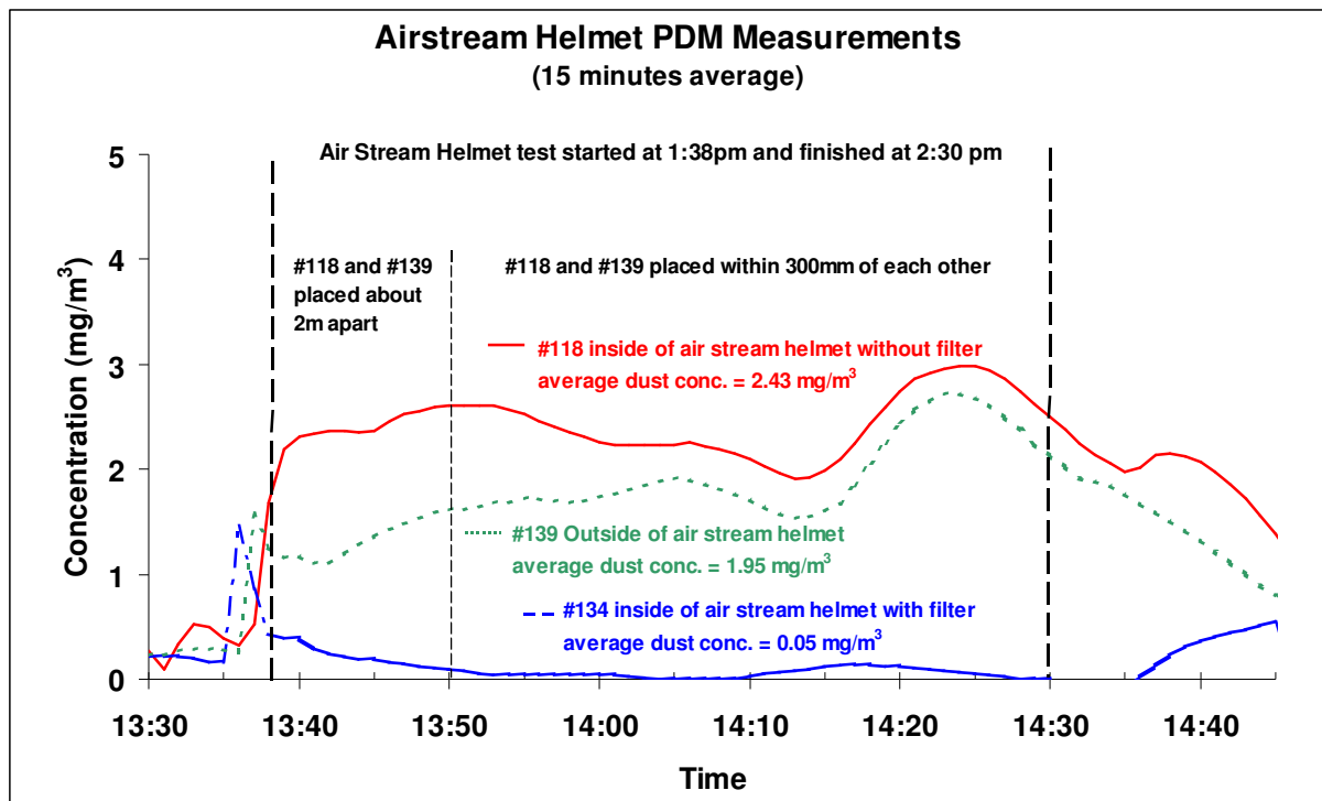
Figure 21 Air steam helmet PDM results
