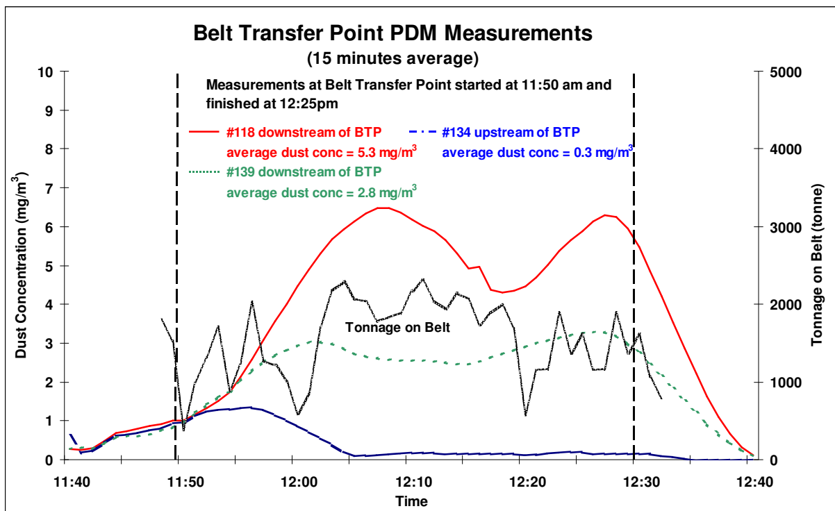
Figure 19 Belt transfer point PDM results.
