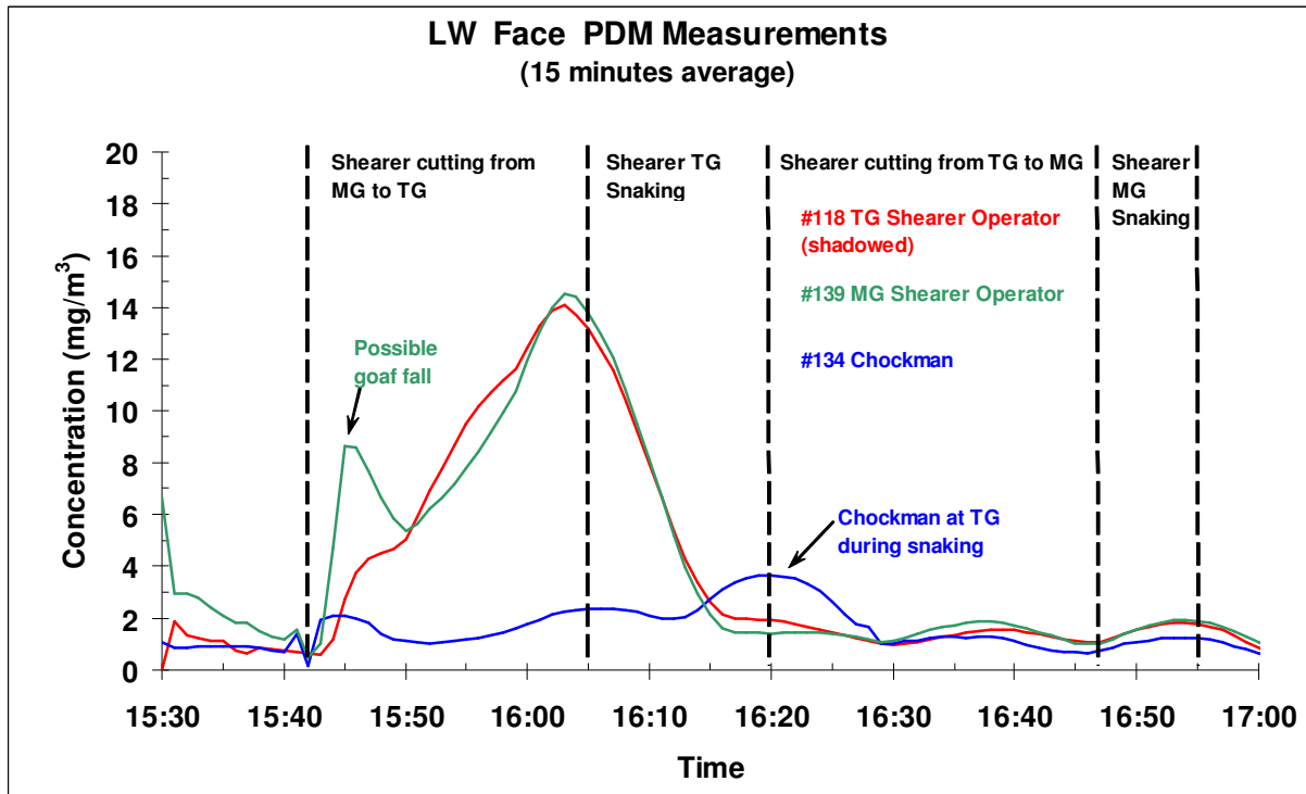
Figure 18 Shearer operators and chockman PDM results under bidirectional cutting.
