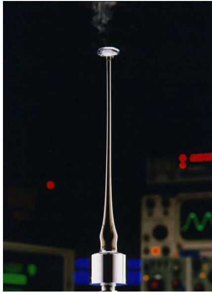
Figure 4 Tapered element with exchangeable filter mounted on narrow end.
