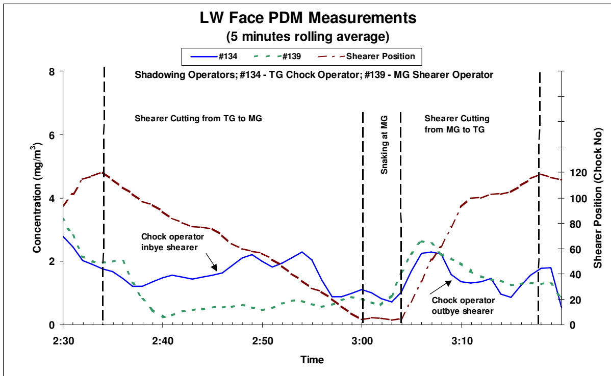
Figure 13 Relative dust make experienced by MG shearer and TG Chock operators.
