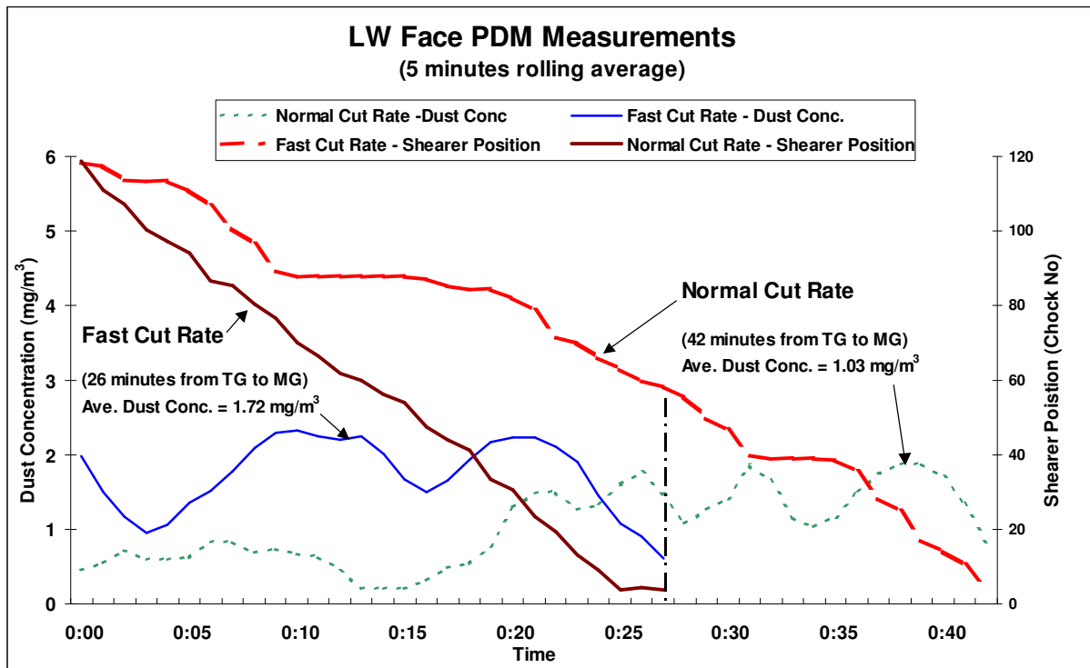
Figure 17 Variation of dust make with shearer advance rates
