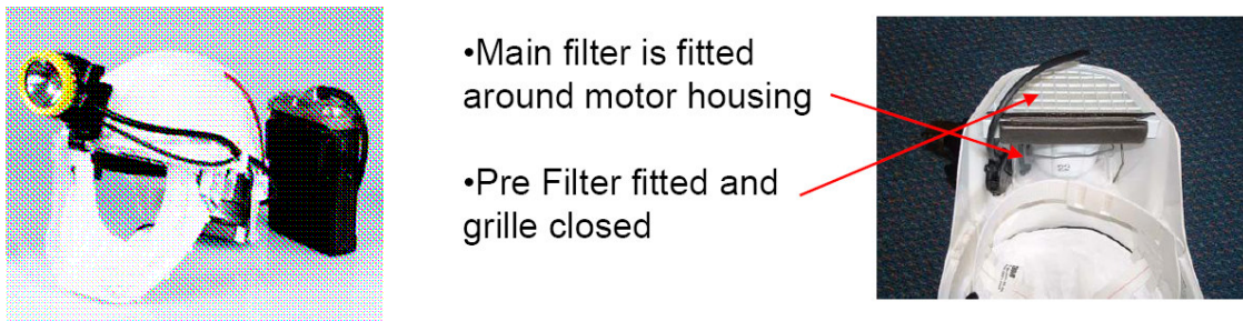
Figure 20 Photographs of air stream helmet and the filters used.
