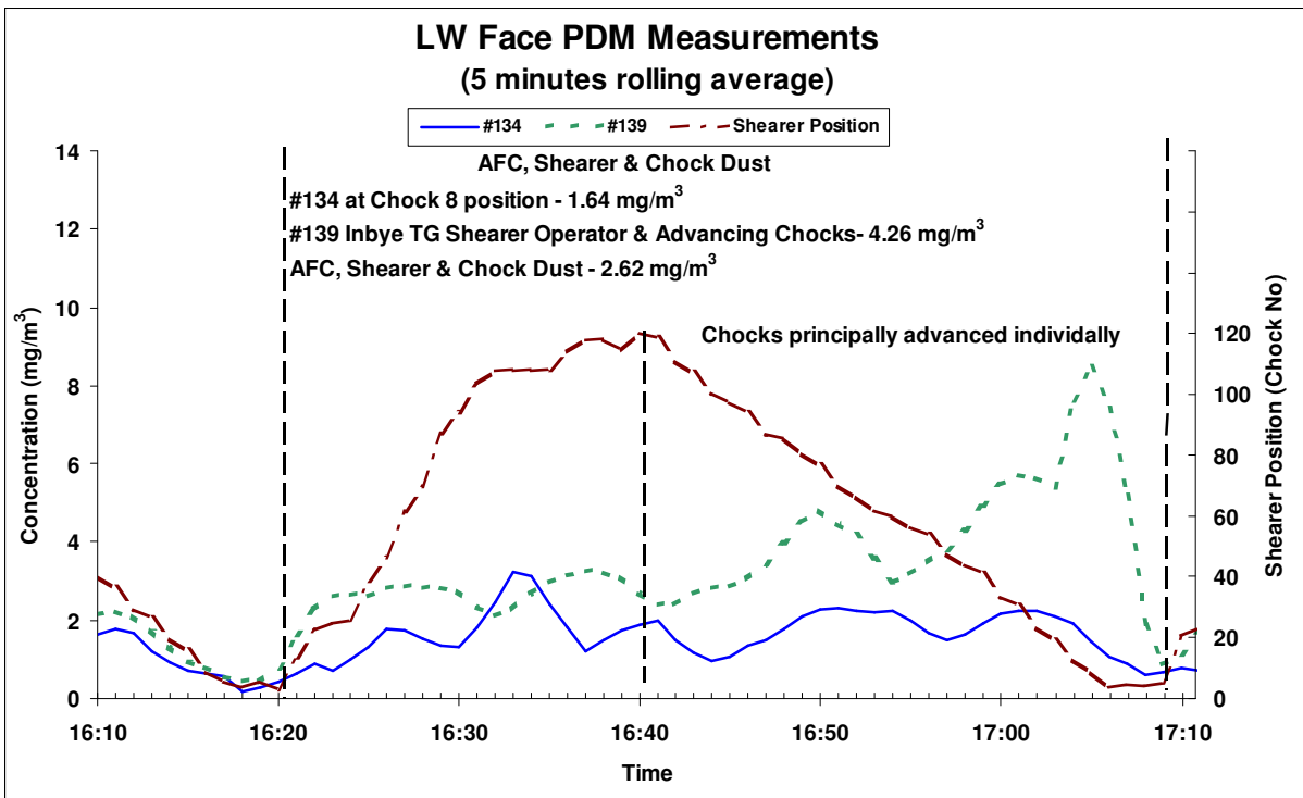
Figure 14 Relative dust make experienced by MG shearer and TG Chock operators.
