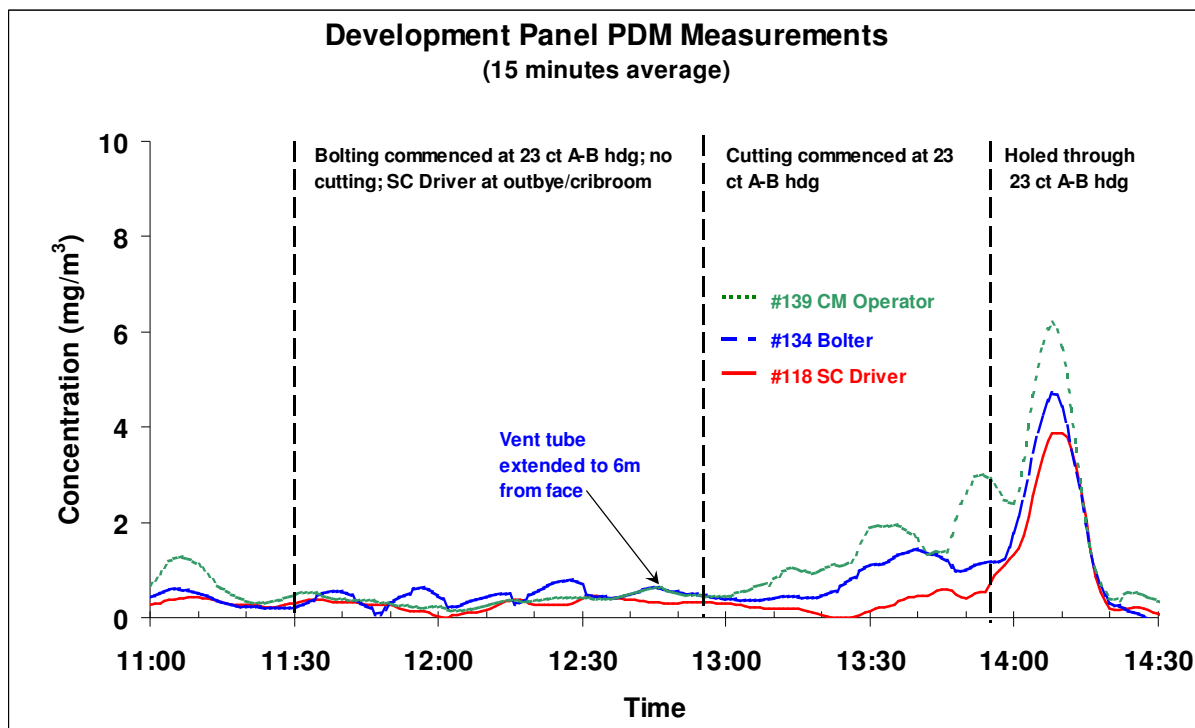
Figure 7 PDM results at development face during cut through holed through.
