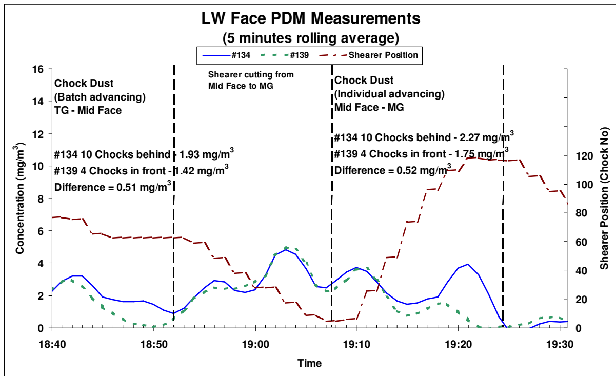
Figure 16 Average dust make from batch and individual chock advance operations.
