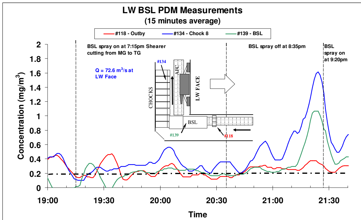
Figure 10 Dust make across a Longwall BSL PDM results – 15 minute average.
