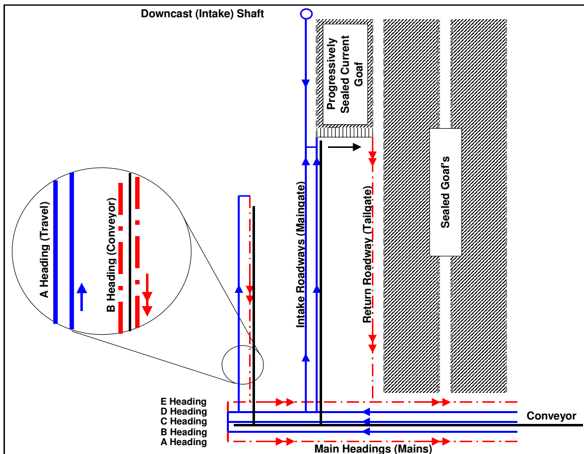
Figure 1. Typical Layout Aspects of Australian LW Mining
