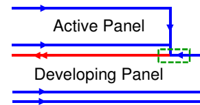
Figure 8 Development air with mixing chamber
