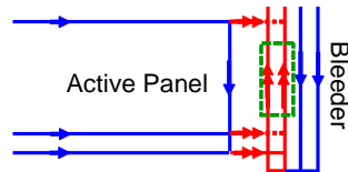
Figure 7 - "Z" LW ventilation with mixing chamber
