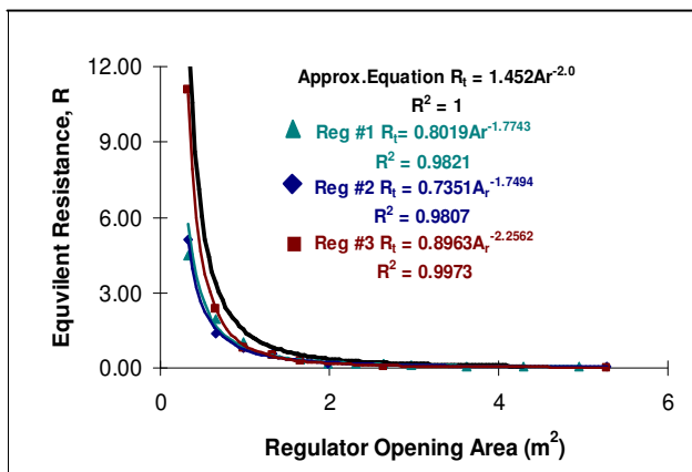
Figure 6 Relationship between R_t and A_r for C-section regulators.
