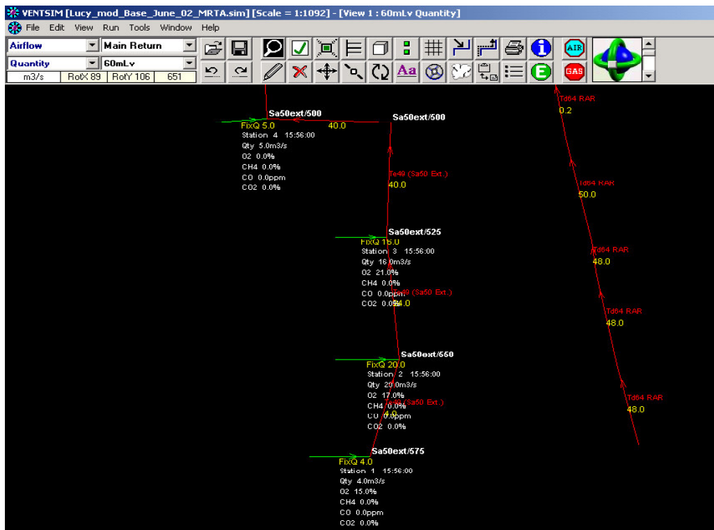
Figure 16 Snap shot of the real time “Ventsim” model at Cannington Sa50 RAR lower levels
