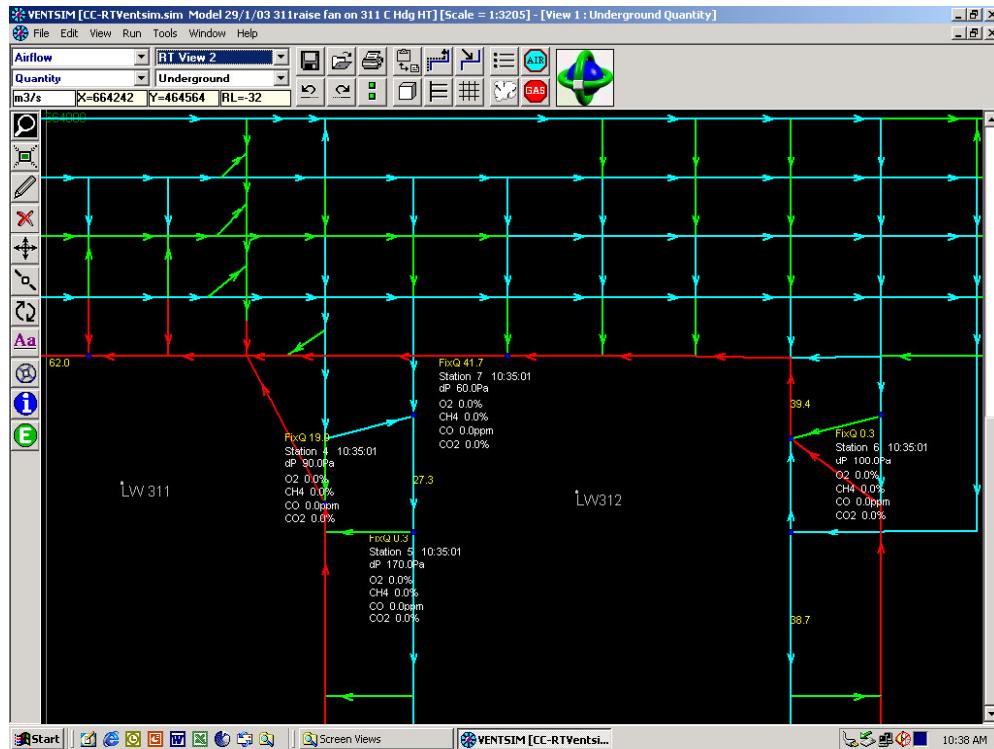
Figure 14 An example of the real time “Ventsim” simulation display at Capcoal Central Colliery
