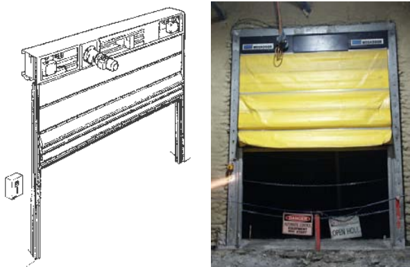
Figure 9 Schematic and photographic views of a roller door regulator
