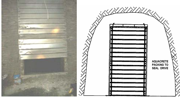
Figure 5 Photographic views and engineering drawing of a half size C-section regulator.
