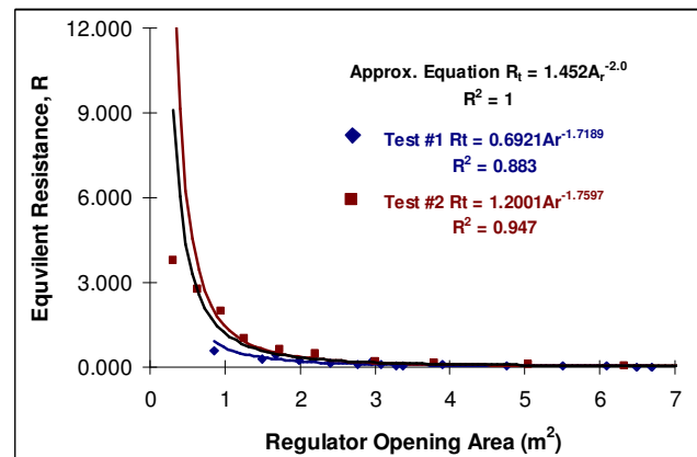
Figure 8 Relationship between R_t and A_r for louvre regulator.
