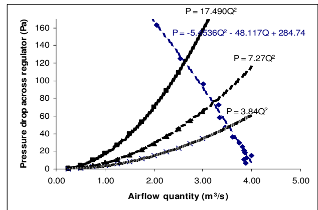
Figure 4. Drop board regulator characteristic curves.
