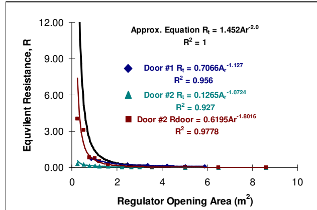
Figure 10 R_t vs. A_r for Roller Door regulator tested
