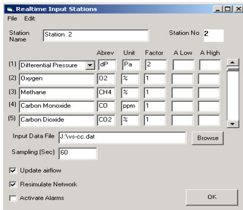
Figure 11 Example of information required for real-time input stations
