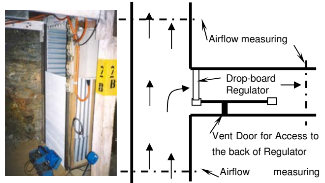
Figure 2. Drop board regulator tested at UQEM.
