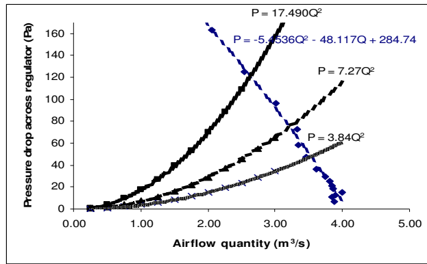
Figure 8. UQEM regulator characteristic curves.
