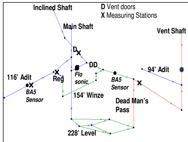
Figure 10 Schematic diagram of UQEM ventilation system.
