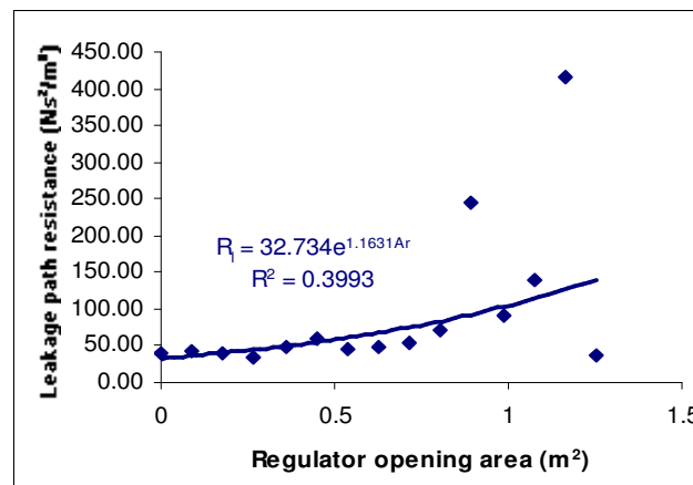
Figure 5. Quantification of resistance for leakage paths.
