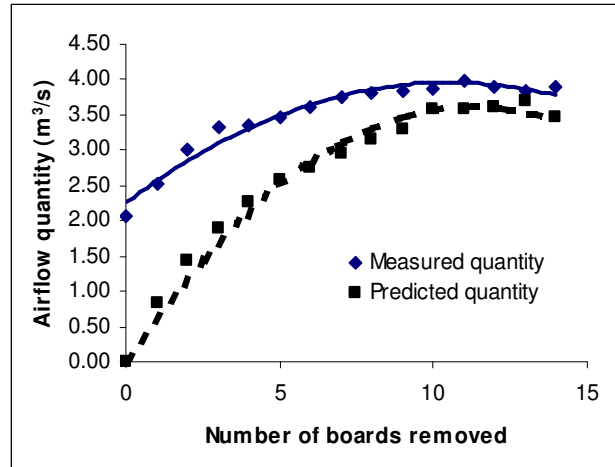
Figure 3. Comparison between measured and predicted quantity.
