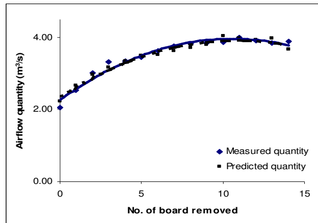
Figure 6. Comparison between measured and new predicted quantity.
