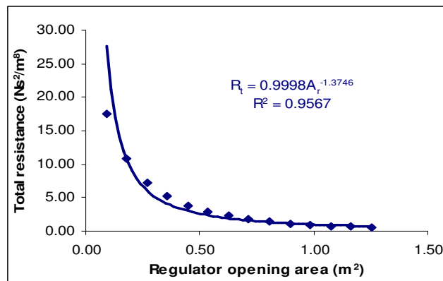
Figure 7. Relationship between new total resistance and regulator opening area.
