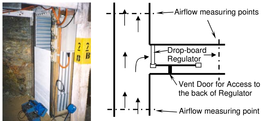
Figure 2. Drop board regulator tested at UQEM.
